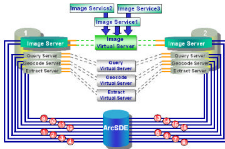
ArcSDE Connections Needed for Three Image Services That Also Reference Geocoding and Data Extraction
