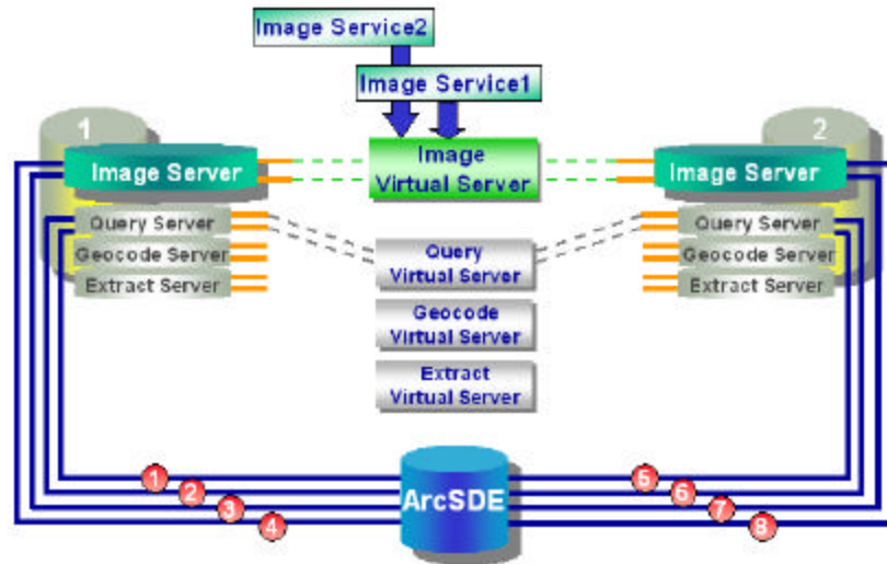
ArcSDE Connections Needed for Two Image Services
