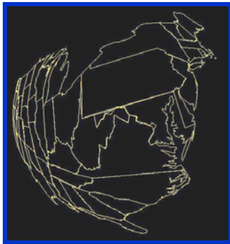
Hyperbolic Geometry
