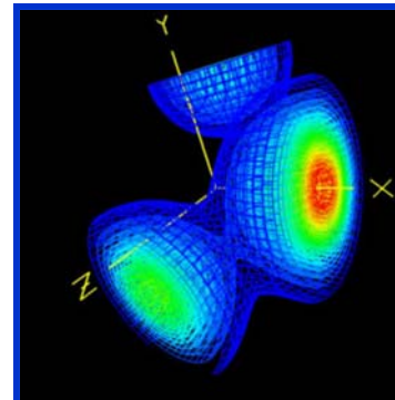
Isosurfaces
